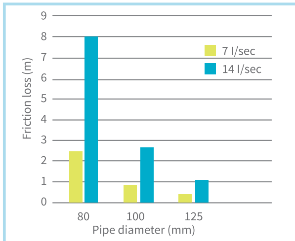
Figure 25 Over stretching the pipe network: doubling the discharge increases the friction (pressure) loss in the system
