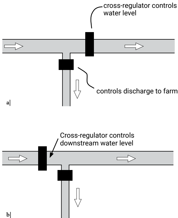
Figure 10 a) Upstream and b) downstream control
