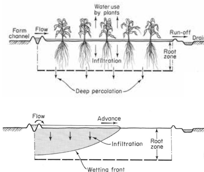
Figure 20 Water movement across the soils surface and in the soil profile during surface irrigation
