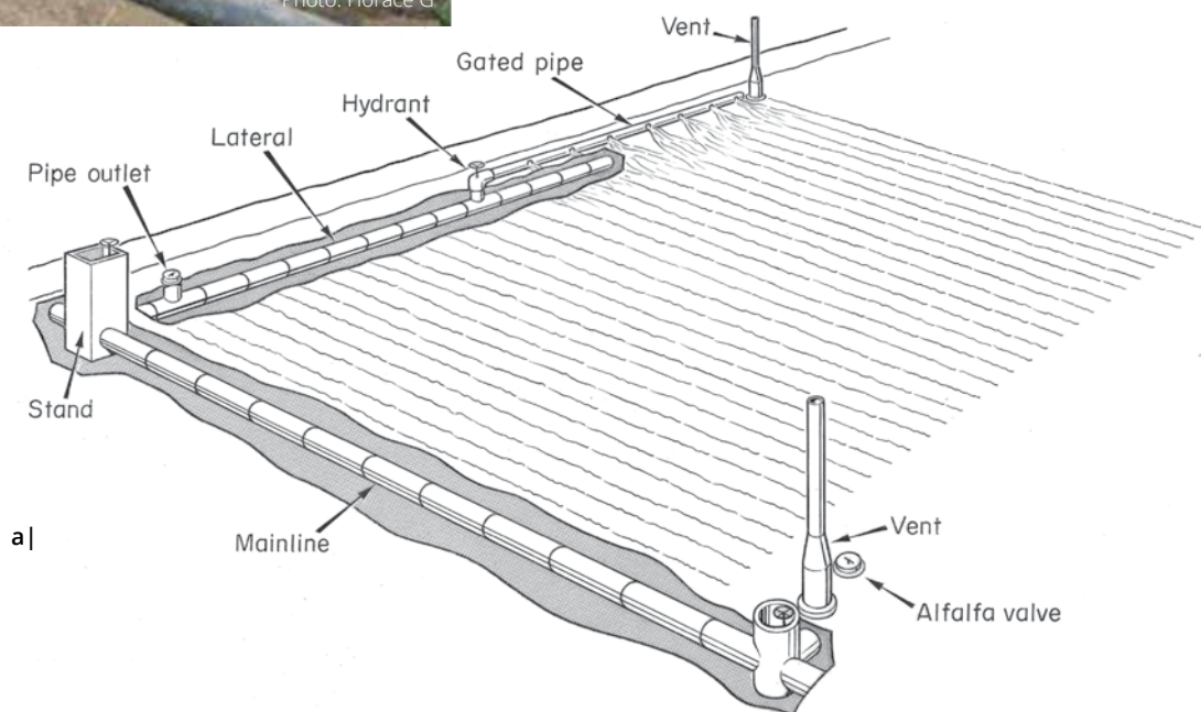
Figure 14 a) Low-pressure pipe system for surface irrigation b) gated pipe used to irrigate furrows.
