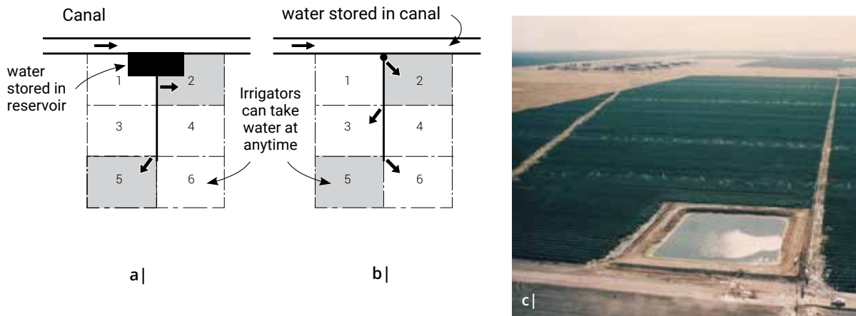
Figure 13 Reservoir storage a) on-farm b) in the tertiary canal c) on-farm reservoir
