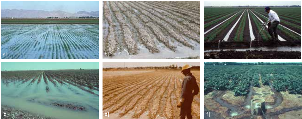
Figure 22 Typical a) basin, b) border, c) furrow irrigation. d) a lack of furrow tail drainage, e) good tail drainage/reuse, f) piped furrow irrigation
