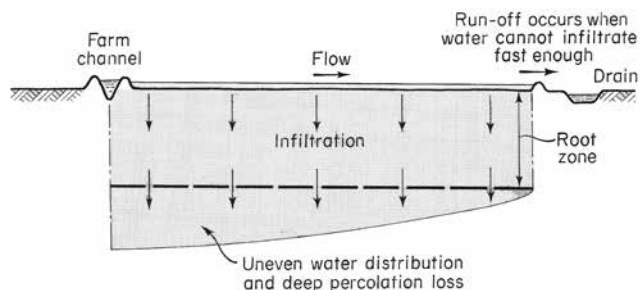
Figure 21 The surface irrigation problem
