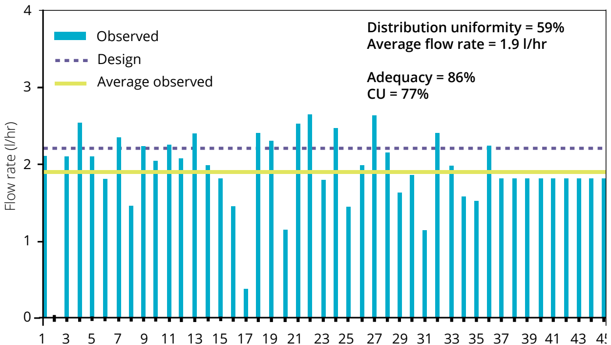
Figure 29 Emitter flow rates measured along a drip line which was two years old.
