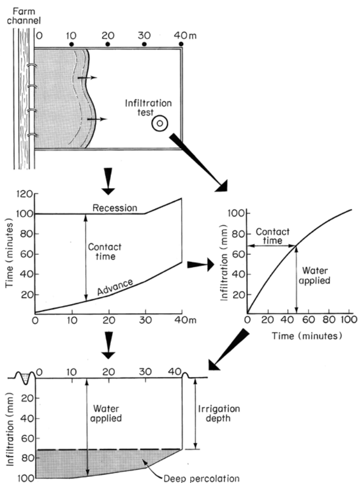
Figure 23 Typical results from a basin irrigation evaluation [55]
